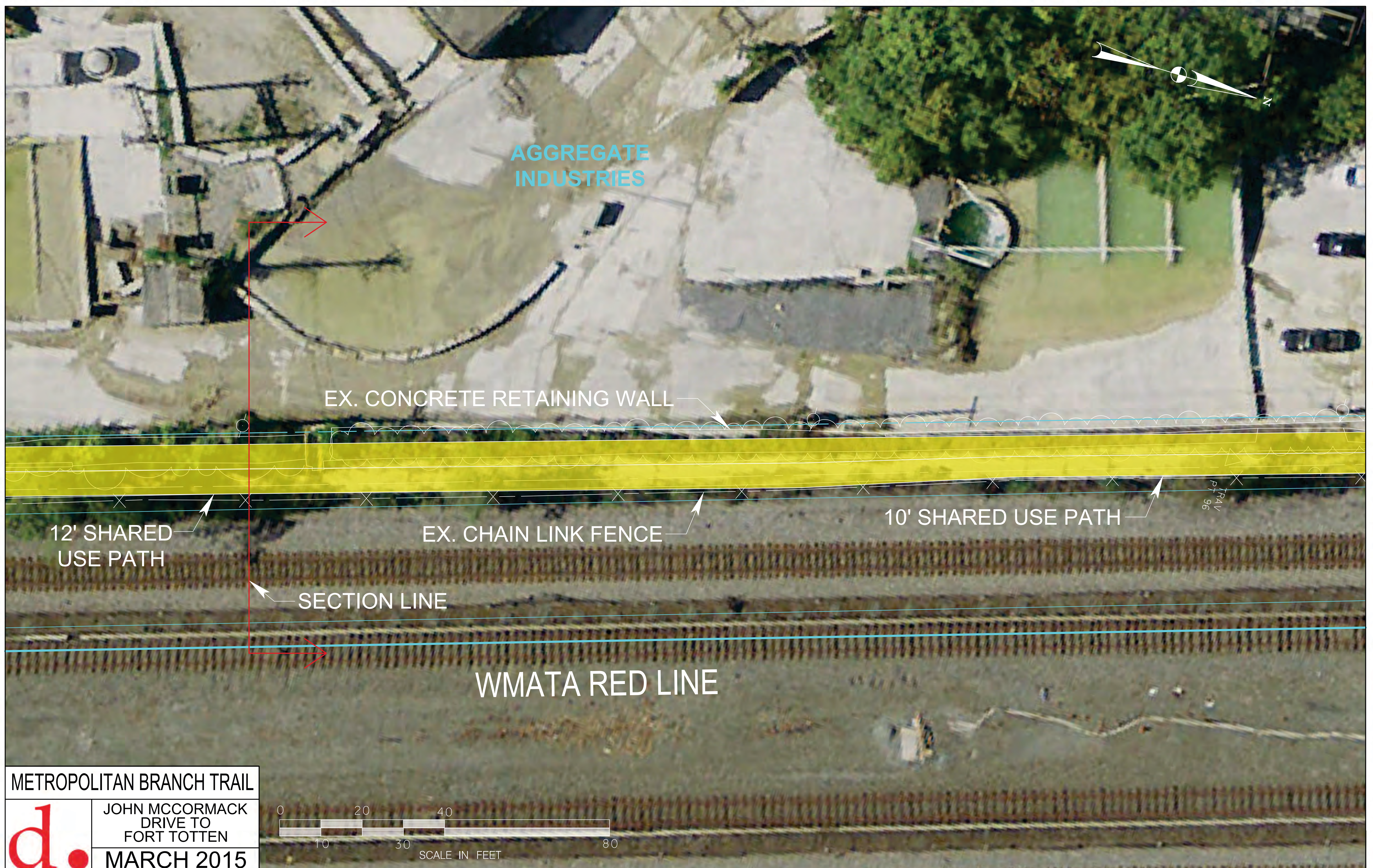
EXISTING CONDITIONS
